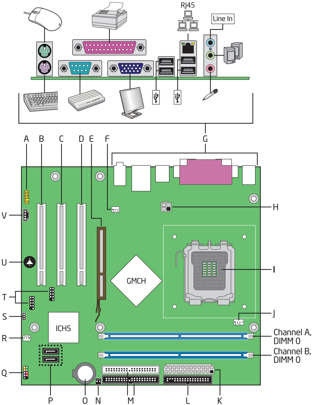
Figure 1. Desktop Board D865GSA Components
